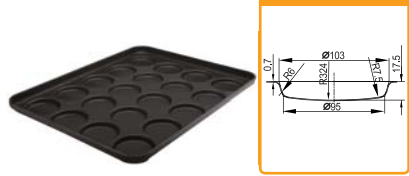
S0810015 4" Hamburger Bun Pan - 20 Impressions
