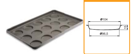
S0710020 Hamburger Bun Pan - 15 Impressions
