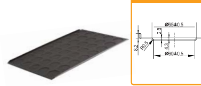
S0610058 Hamburger Bun Pan - 40 Impressions
