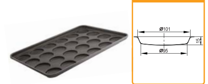
S0610046 4" Hamburger Bun Pan-24 Impressions
