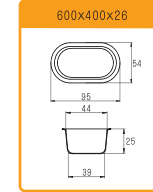
SN9089 Oval Bread Mould-36 Indents (Non-stick)
