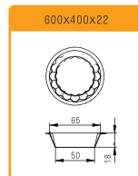
SN9302 Briochette Mould-35 Indents (Silicone)
