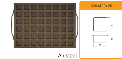
SN9070 Pineapple Cake Mould-48 Indents (Non-stick)
