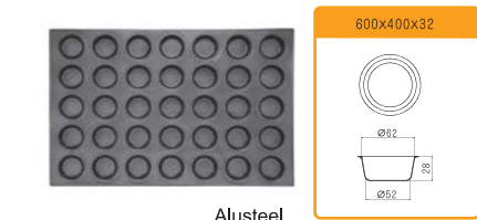
SN9088 Muffin Mould-35 Indents (Silicone)
