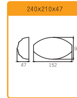
SN9014 2 Straps Bomb Mould (Non-stick)
