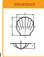
SN9035 Madeleine Mould-28 Indents (Silicone)
