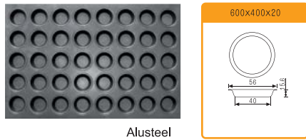
SN9075 Tart Mould-40 Indents (Non-stick)
