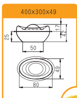
SN9132 16 Straps Gold Ingot Cake Mould (Non-stick) Patent No.:ZL201120196179.4
