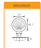
SN9047 Madeleine Mould-11 Indents (Silicone)
