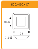
SN9131 Square Cake Mould-35 Indents (Silicone)
