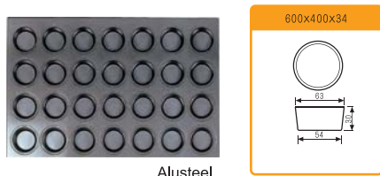
SN9084 Muffin Mould-28 Indents (Silicone)
