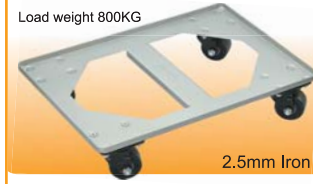
Steel Trolley(Spray Paint) SN1982 610x410x125
