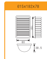
SN9113 6 Straps Crimped Round Bread Mould (Non-stick)
