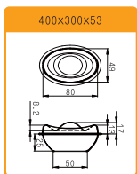
SN9134 16 Straps Gold Ingot Cake Mould(Silicone)
