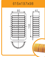
SN9116 6 Straps Crimped Round Bread Mould (Non-stick)
