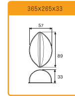
SN9026 Lemon Cake Mould-9 Indents (Silicone)
