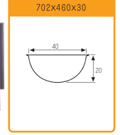
SN9100 Half Sphere Bread Mould-60 Indents (Non-stick)
