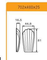
SN9045 Madeleine Mould-35 Indents (Silicone)
