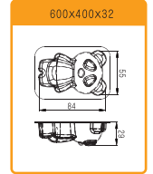
SN9092 Panda Cake Mould-25 Indents (Silicone)
